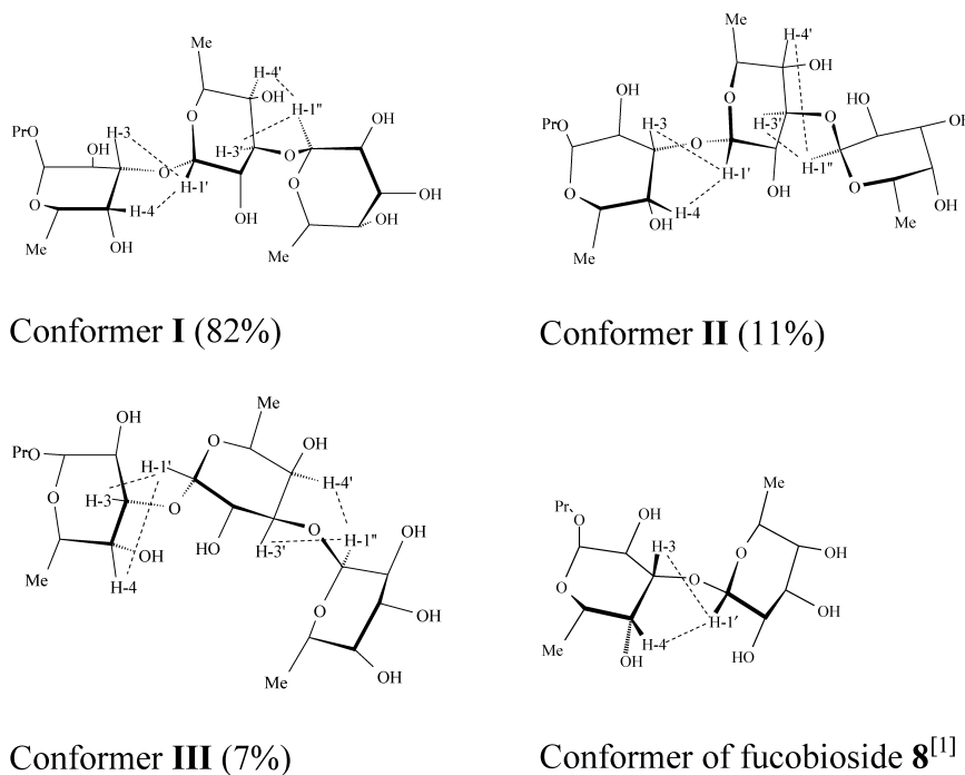
Figure 3. Conformers of the non-sulfated trisaccharide 1 with their statistical weights and schematic representation of one of the conformers of the related fucobioside 8 [1] .
